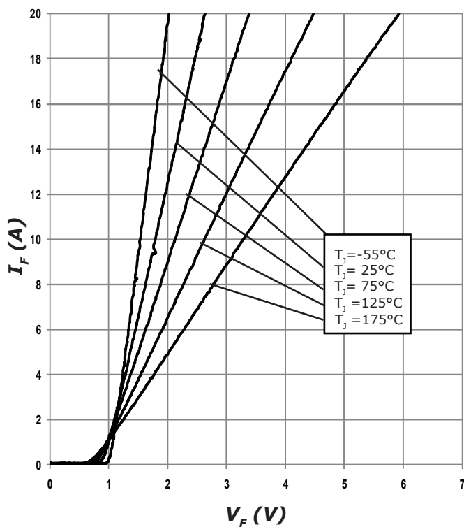
Figure 1. Forward Characteristics
